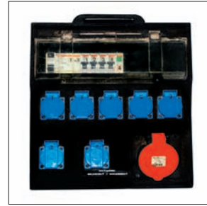
Electrical panel 380V/220V Code 019.010.265.000 EUR 120.00
